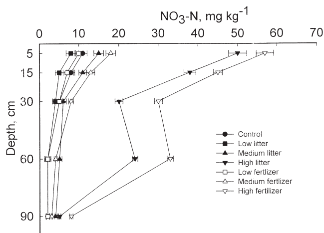
Fig. 2. Effects of broiler litter and commercial fertilizer application rates on postharvest residual soil \text{NO}_3\text{-N} in 2002.
